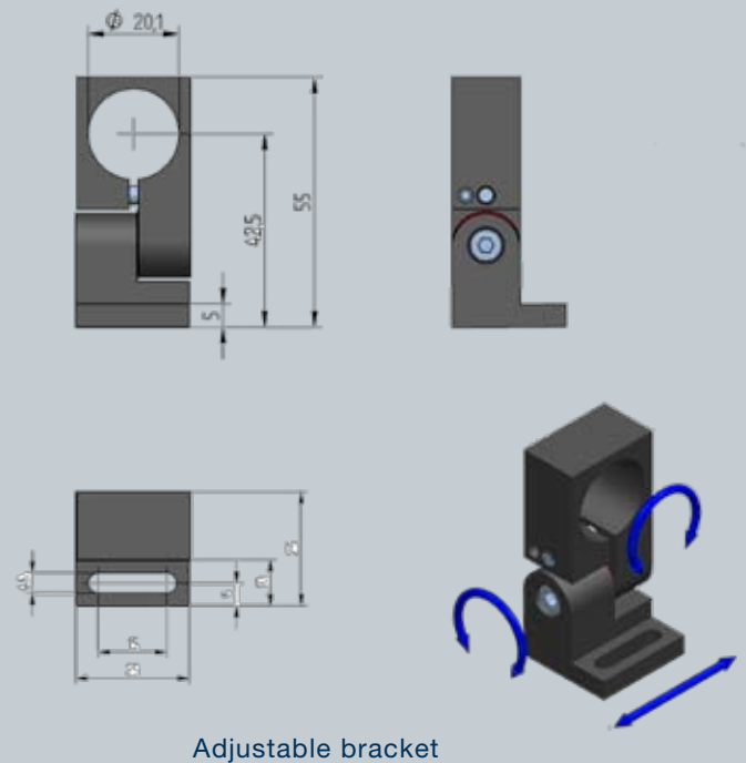
Adjustable bracket
